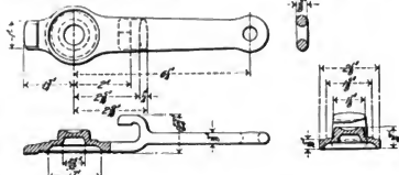
Figs. 2973-2976. Signal Hose Dummy Coupling.
